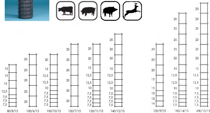
Ursus Heavy
