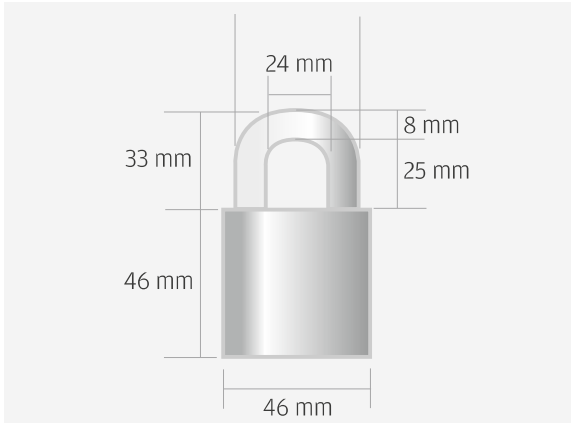
Recommended padlocks.
